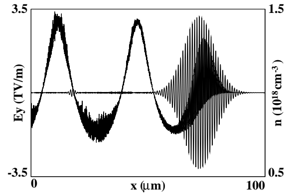
Figure 1: One-dimensional diagram of photon acceleration. Shown are the profiles of electron density (dark line) and propagating laser pulses.
